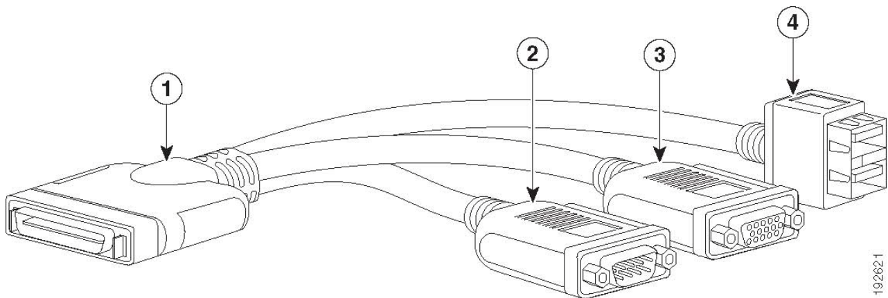
Figure 19 KVM Cable
