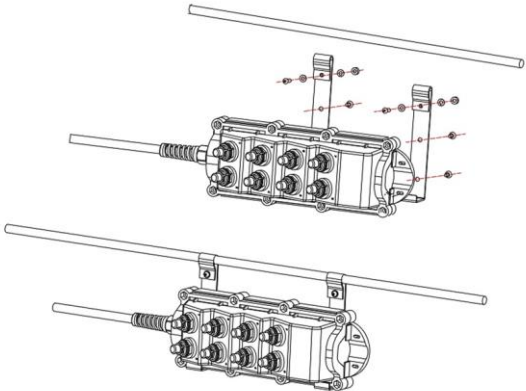
Aerial Installation
